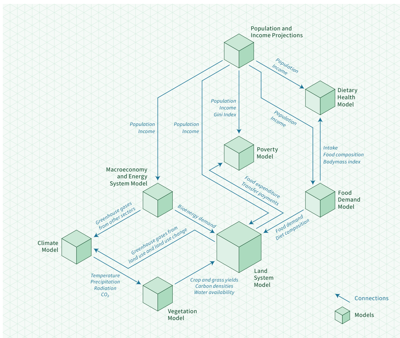
FIGURE 2.2 Modeling Framework
